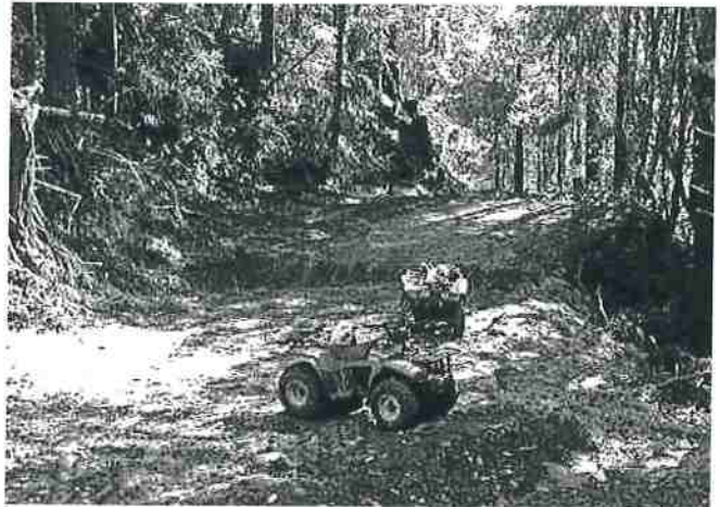
Figure 9. Water bars installed on a road after timber harvesting. Source: Angela Wilson, Central Valley Regional Water Quality Control Board.
