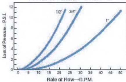
Head Loss Curves - 1/2", 3/4", 1"
