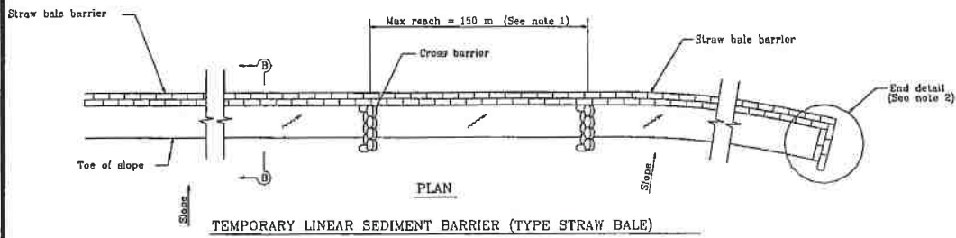
TEMPORARY LINEAR SEDIMENT BARRIER (TYPE STRAW BALE)
