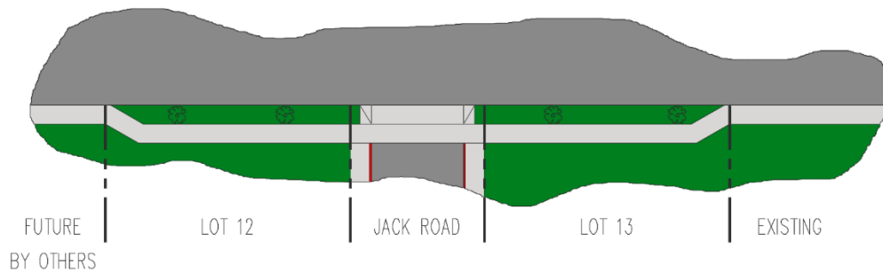
Above: Plan view of Gwin Road widening and Jack Way intersection
