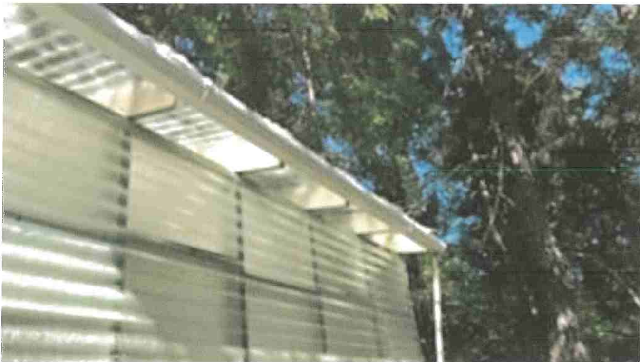
Rain gutter on shed roof and drain pipe to irrigation line
