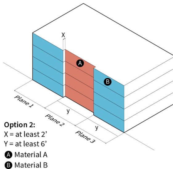
Figure 2-43: Minimum 2x6' Break with Material Change
