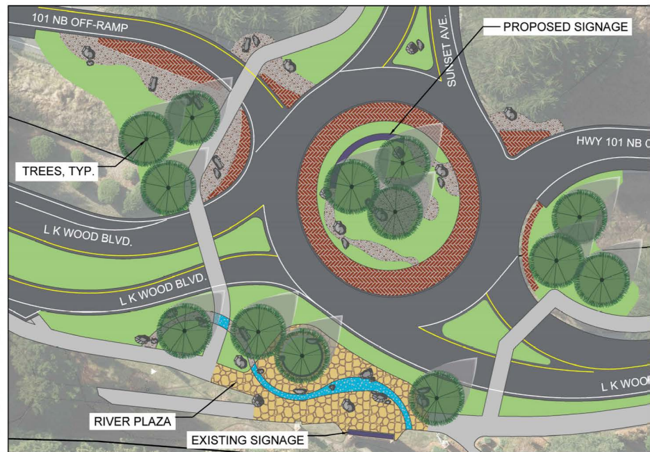
L K WOOD BOULEVARD ROUNDABOUT PLAN OVERVIEW
