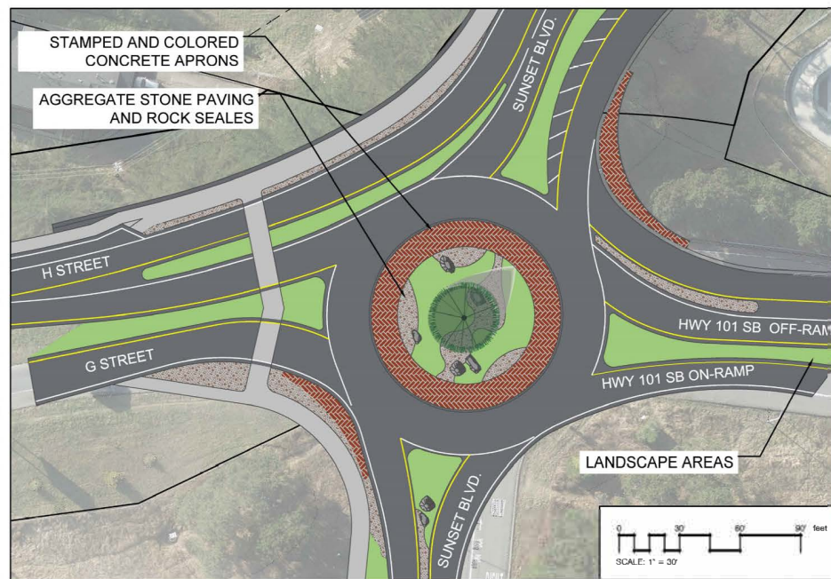
H STREET ROUNDABOUT PLAN OVERVIEW
