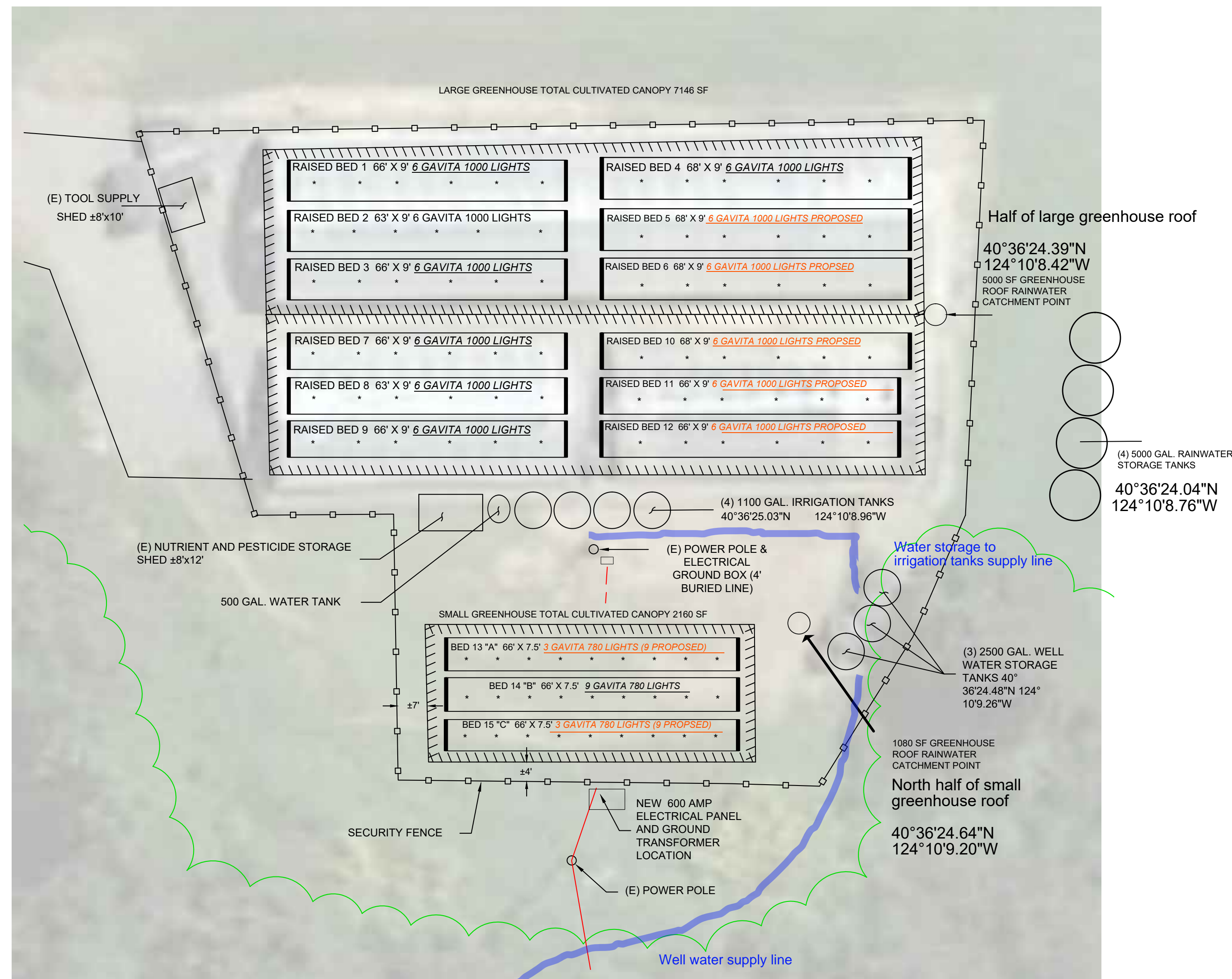
GREENHOUSE PLAN DETAIL
