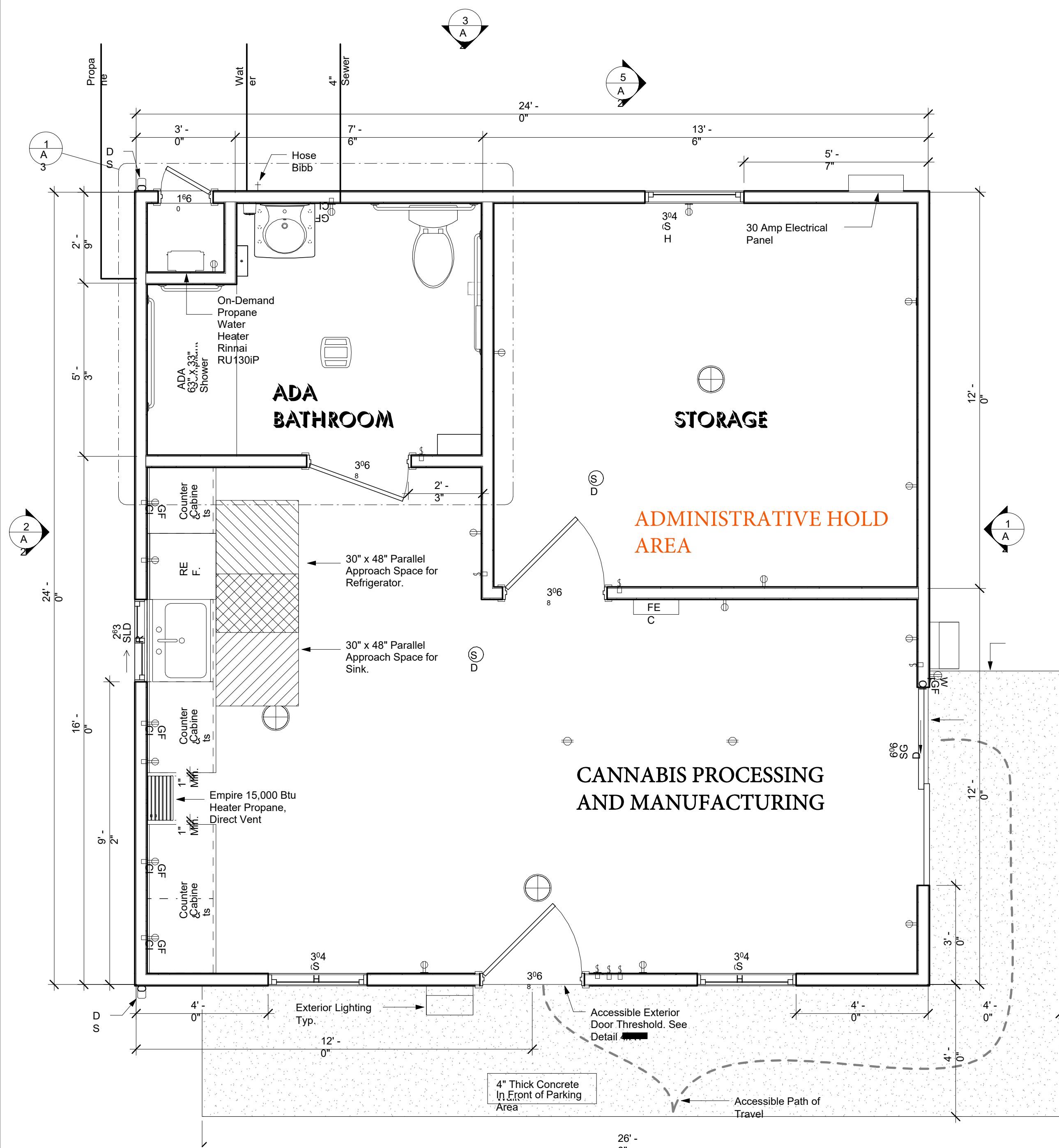
PROCESSING ROOM DETAIL
