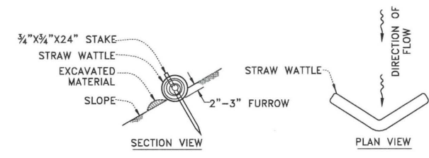
STRAW WATTLE DETAIL NOT TO SCALE
