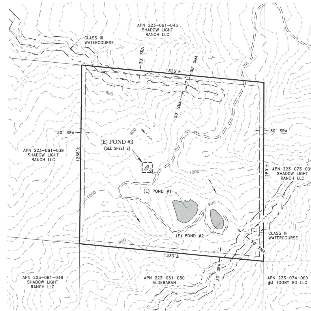
SITE PLAN SCALE: 1" = 400' (IF PRINTED AT 11x17)
