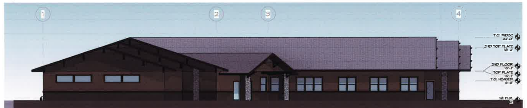
2 SOUTH 1" = 10'-0"
