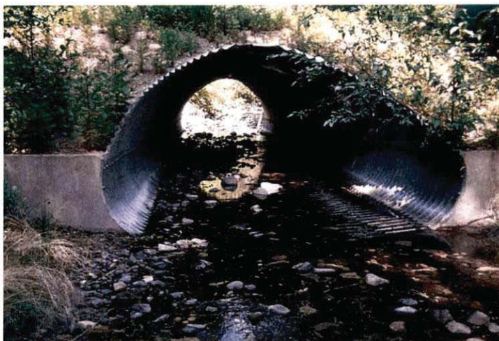
Figure 28. An arched pipe installed on a fish-bearing stream to minimize impacts on fish habitat and migration. Source: Keller and Sherar 2003.
